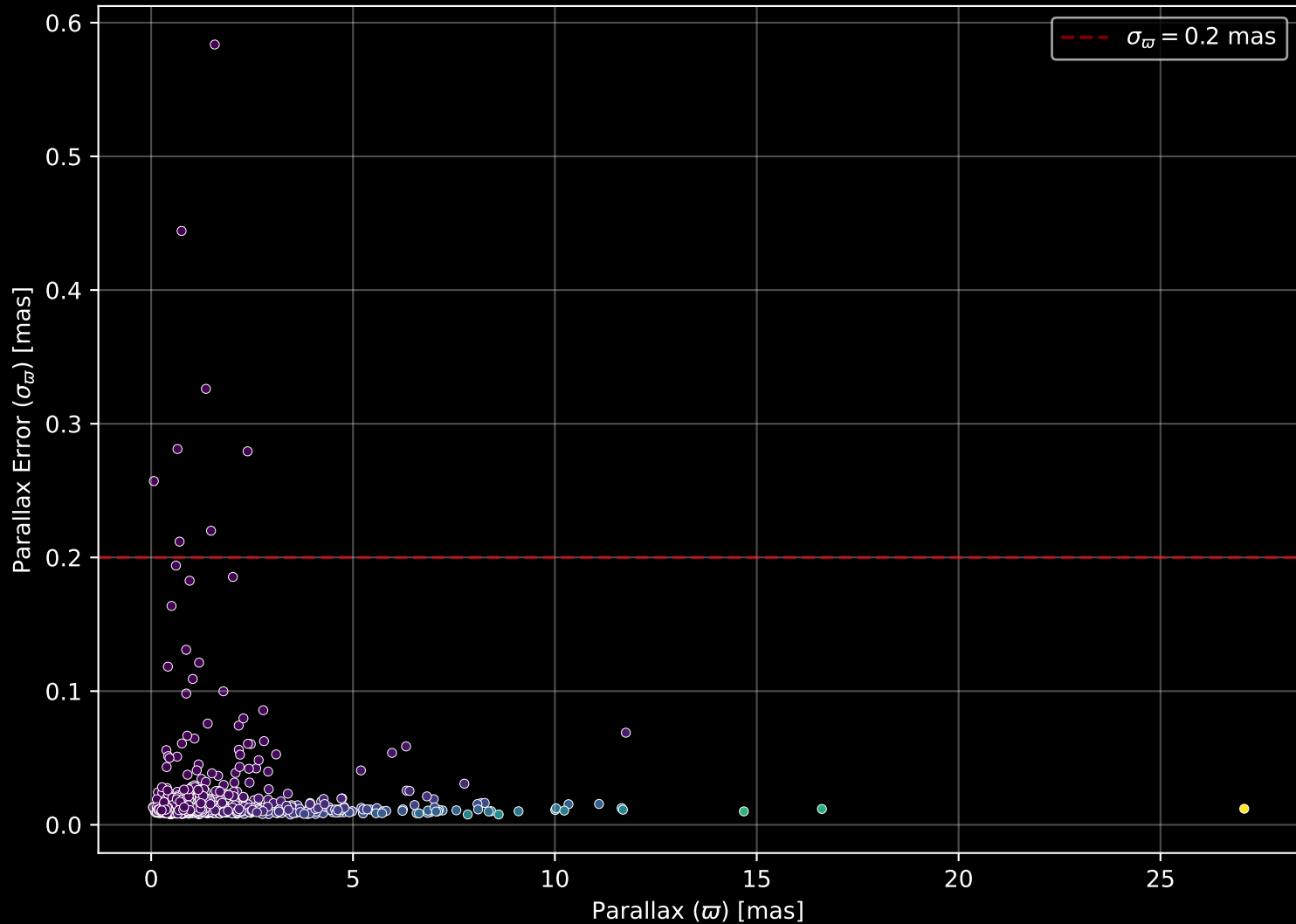
APOGEE DR17 Field: [K10_079+12] Parallax Quality (n= 881)
