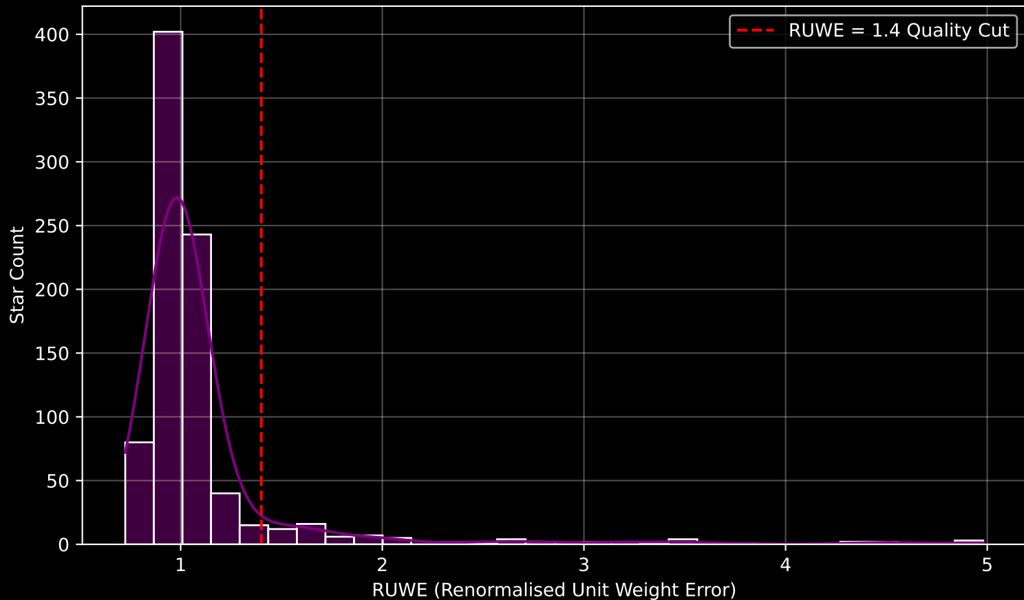
GAPOGEE DR17 Field [K10_079+12] RUWE Distribution (n= 854)
