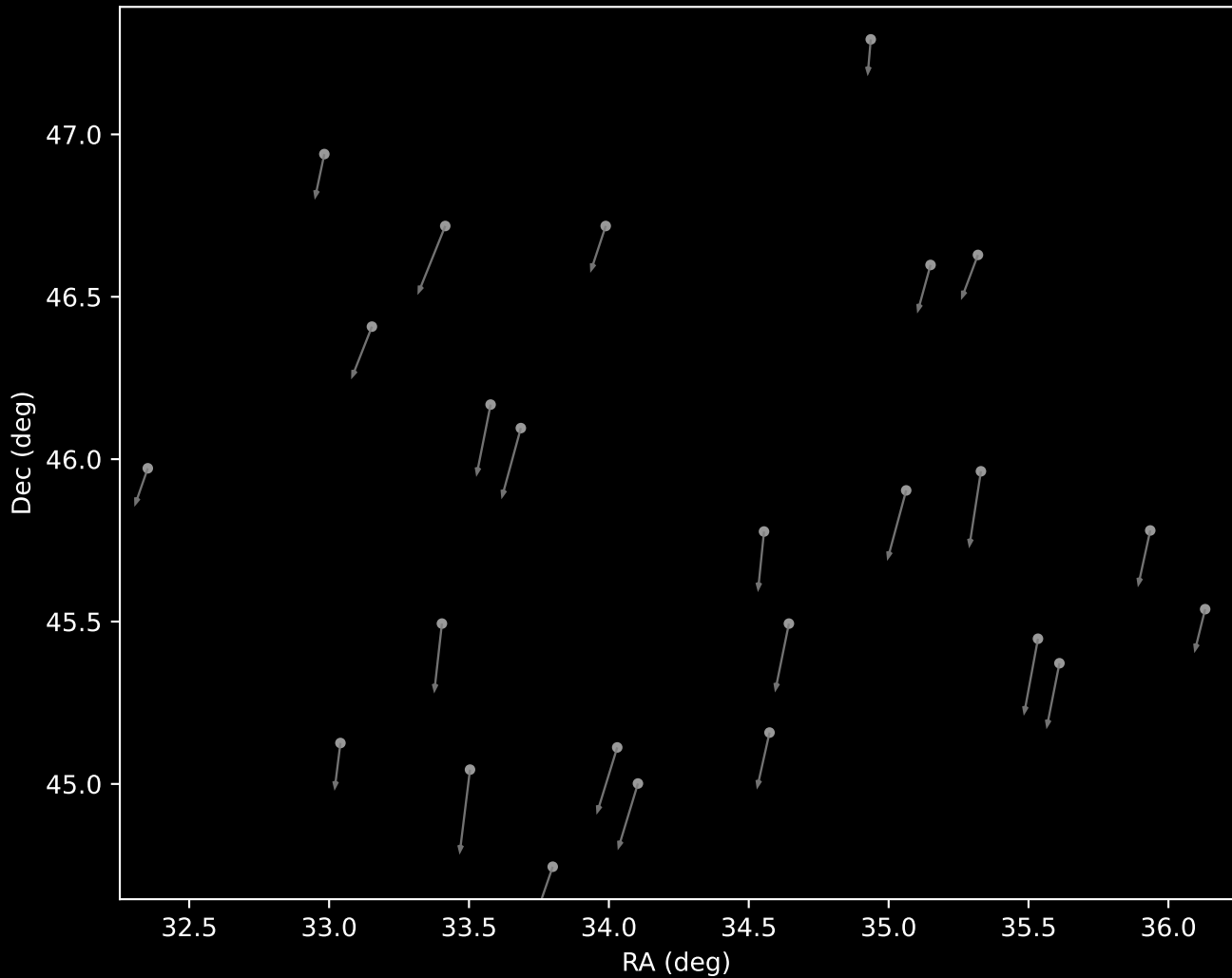
APOGEE DR17 Cluster 14 Proper Motion Vectors (n=25)
