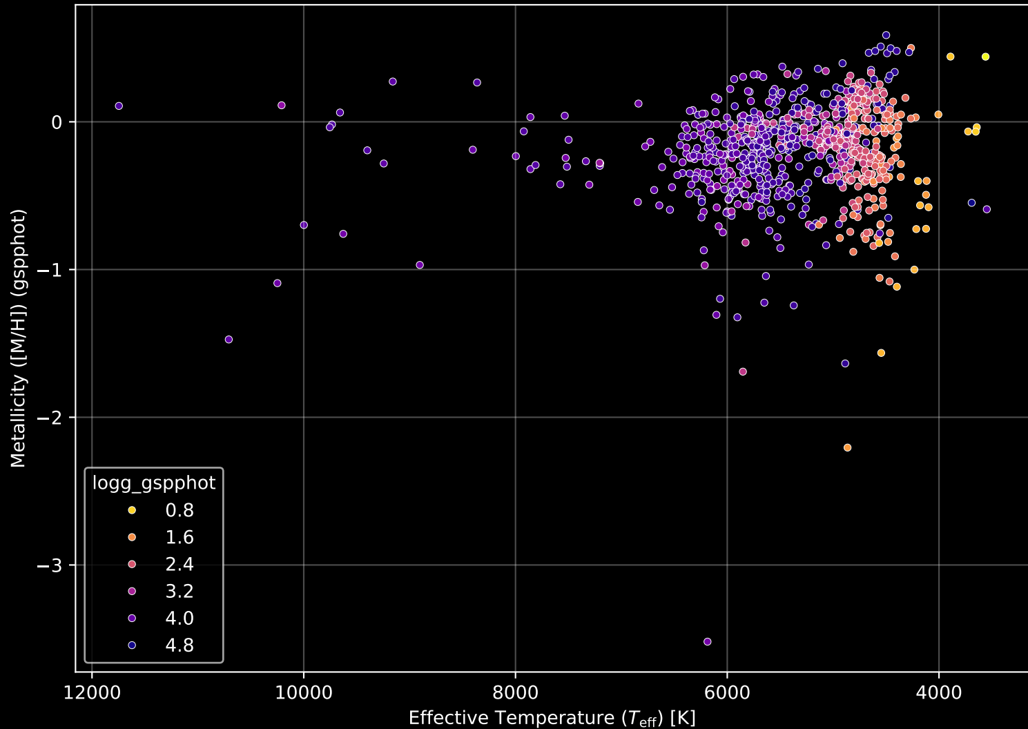
APOGEE DR17 Field: [K10_079+12] Stellar Population Parameters (n= 881)
