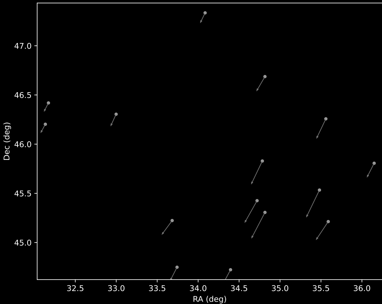
APOGEE DR17 Cluster 34 Proper Motion Vectors (n=15)
