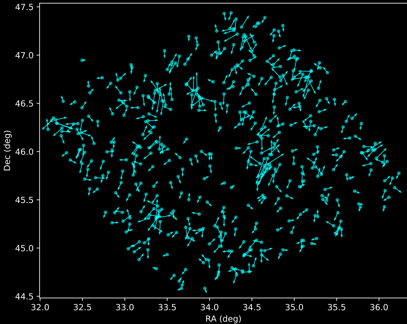
APOGEE DR17 Noise Stream Proper Motion Vectors (n=457)
