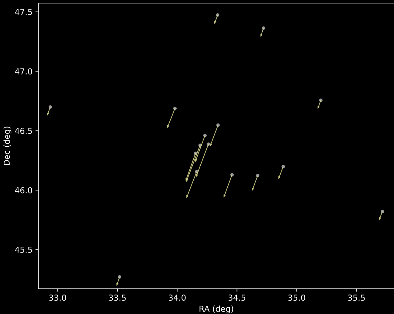
APOGEE DR17 Cluster 37 Proper Motion Vectors (n=16)
