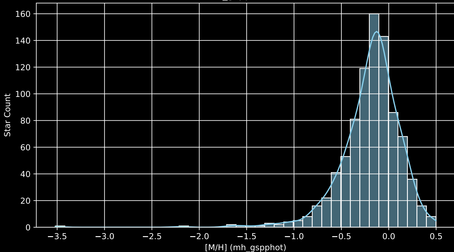
APOGEE DR17 Field: [K10_079+12] [M/H] (mh_gspphot) (n= 878)
