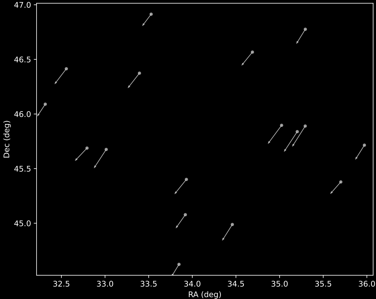
APOGEE DR17 Cluster 35 Proper Motion Vectors (n=17)
