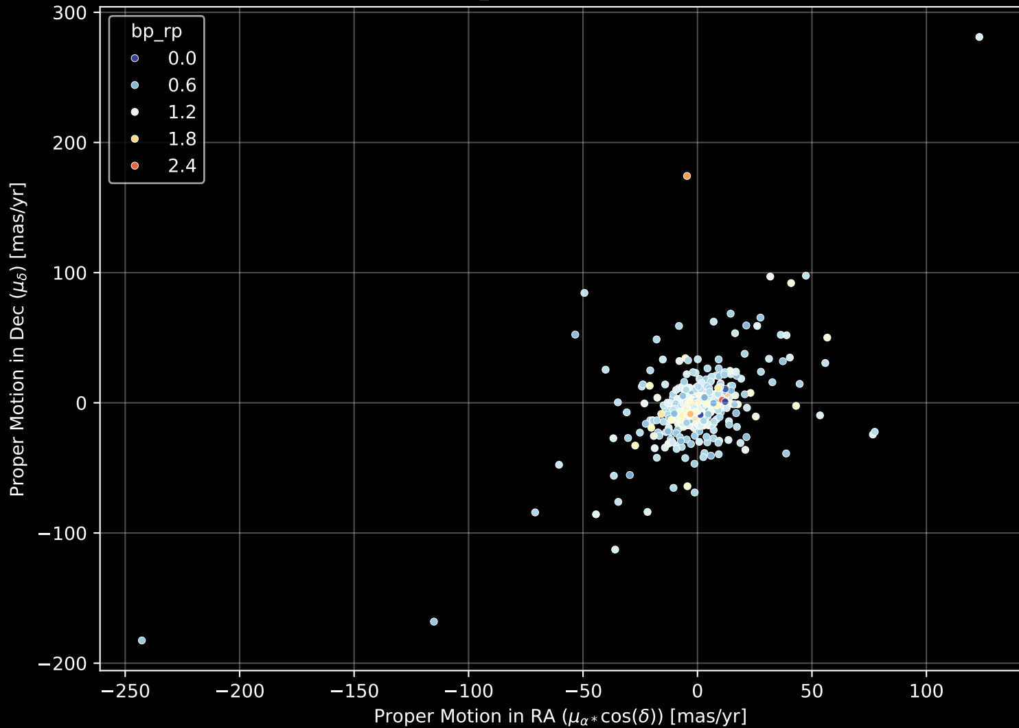
APOGEE DR17 Field: [K10_079+12] Proper Motion Diagram (n= 881)
