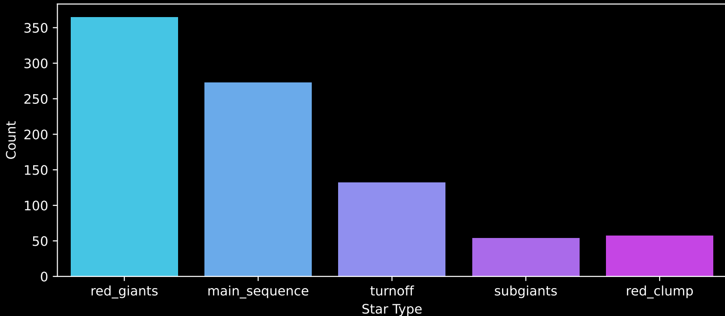
APOGEE DR17 Field: [K10_079+12] Count plot of Star Type
